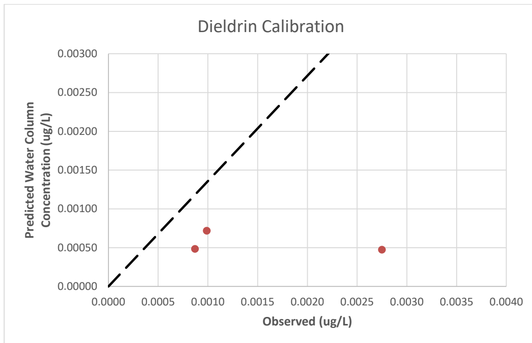
Figure B-1. Diieldrin Calibration Results. Dashed line indicates 1:1 fit between observations and predictions.
